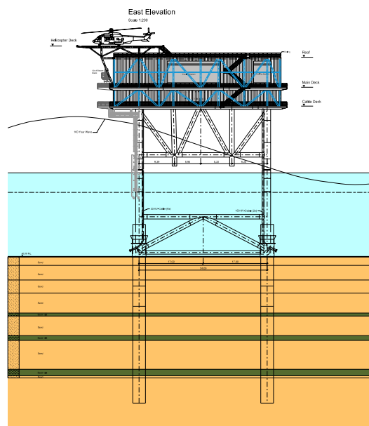
General layout substation “East”
