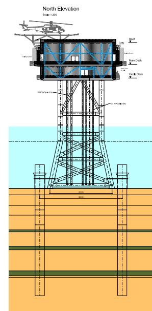
General layout substation “North”
